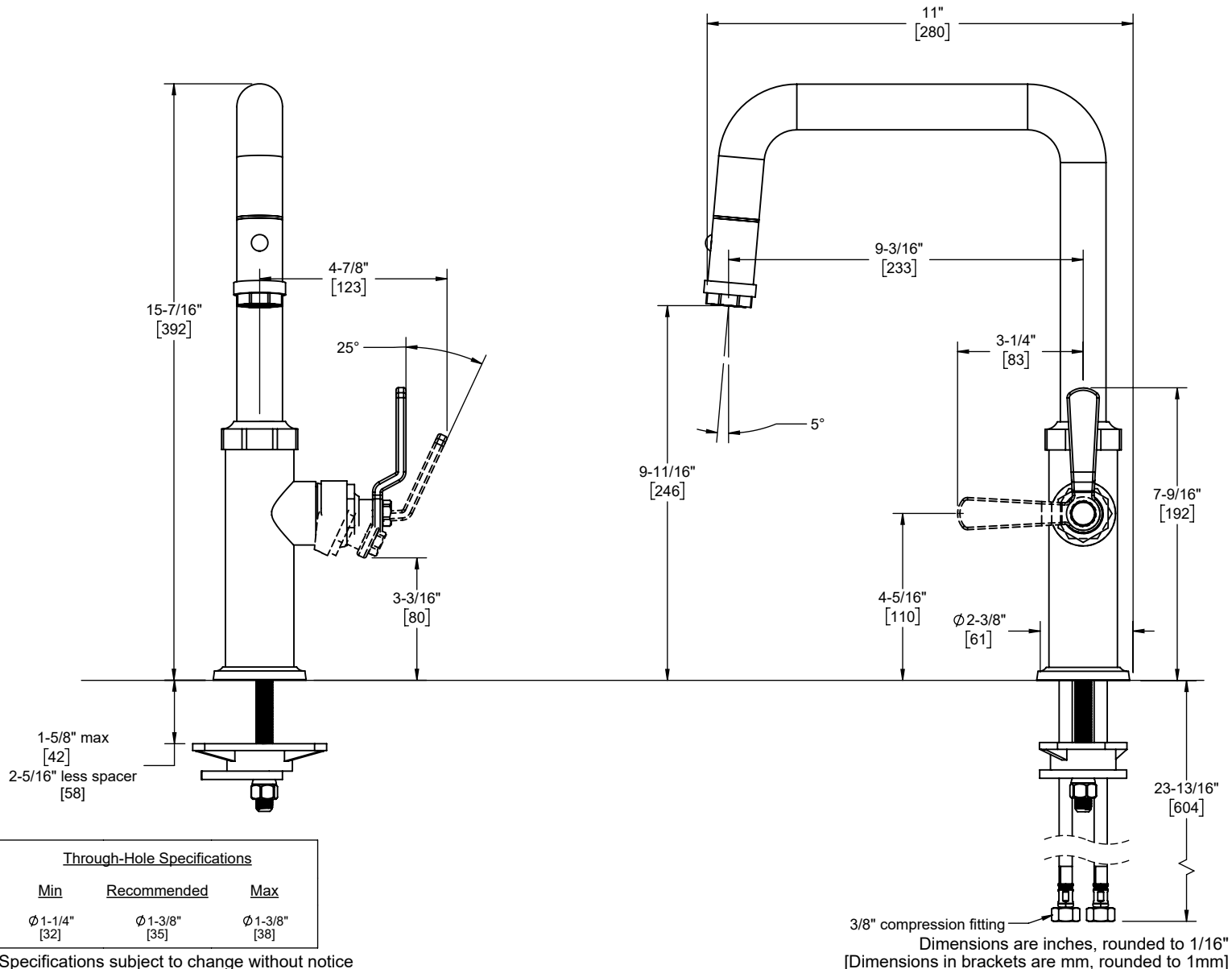
K81-103-BL-ZZ shown
